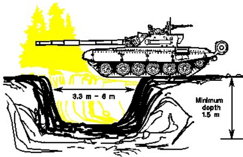
Figure 5-13. Antitank ditch.
